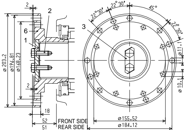
KIT 2.05.405.0000 SPICER 1600/1700/1800
