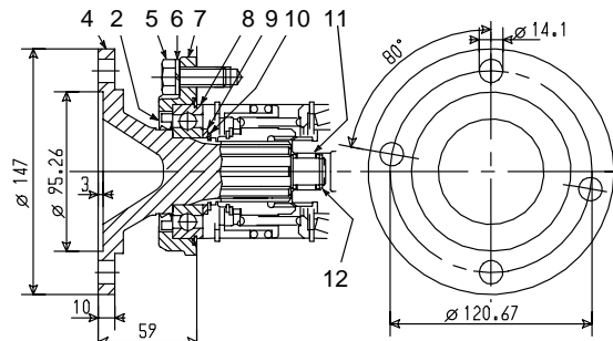
KIT 2.05.364.0000 SPICER 1500
