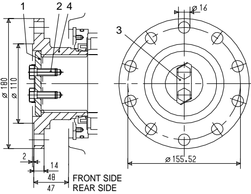
KIT 2.05.405.0000 SPICER 1600/1700/1800
